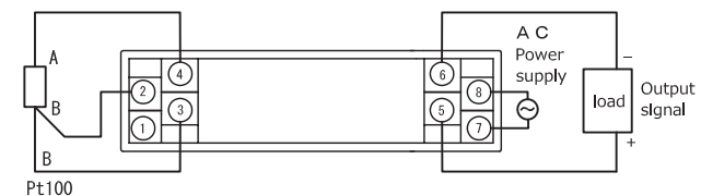
■ Input / output connection diagram
