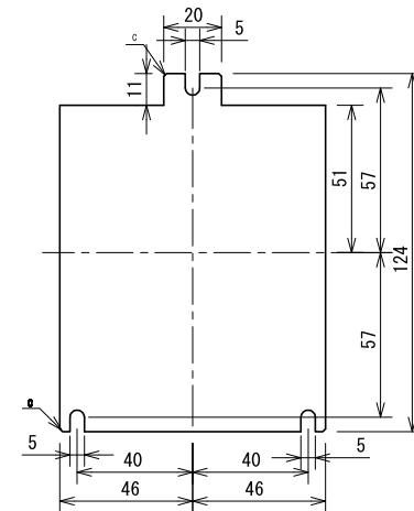
Mounting dimension drawing
